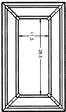
Top View with Lid Removed
